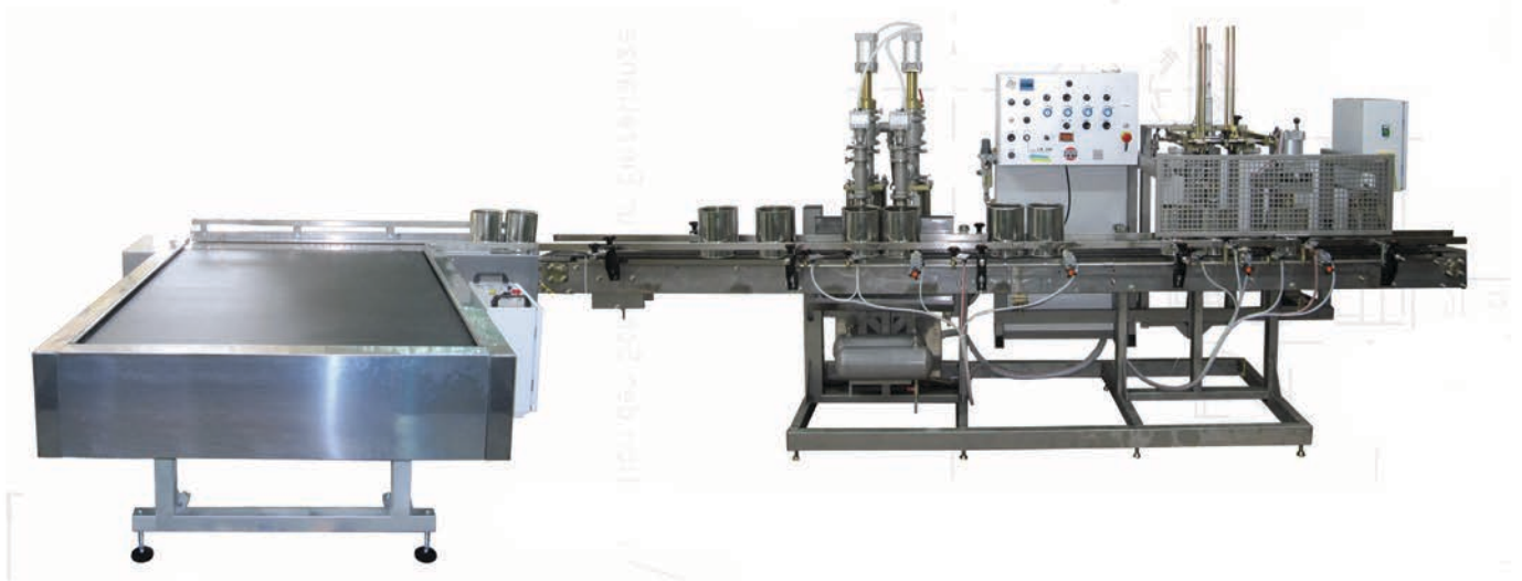
Filling Line LR.2M with rectangular table
