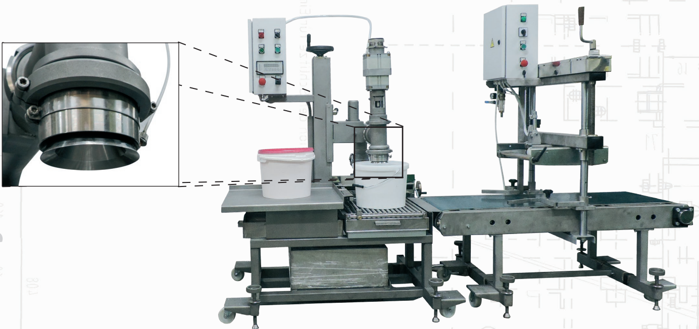
PRK.022 ПРК.022
